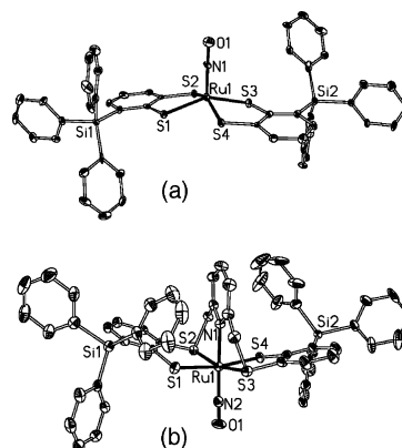
Figure 1. ORTEP diagrams of (a) the anion of 2 and (b) the cation of 3 (50% probability ellipsoids; H atoms and solvent molecules omitted). Selected distances [Å] and angles [°] for 2 : Ru1–N1 1.699(5), Ru1–S1 2.338(2), Ru1–S2 2.321(2), N1–O1 1.195(7), N1–Ru1–S1 108.2(2), N1–Ru1–S2 104.9(2), S1–Ru1–S2 85.43(6), S1–Ru1–S3 148.65(7), S2–Ru1–S4 151.78(7), Ru1–N1–O1 177.4(6). 3 : Ru1–N1 2.099(4), Ru1–N2 1.748(4), Ru1–S1 2.393(2), Ru1–S2 2.345(2), Ru1–S3 2.363(2), Ru1–S4 2.371(2), N2–O1 1.144(5), N1–Ru1–N2 178.1(2), N1–Ru1–S1 85.7(2), N2–Ru1–S1 96.2(2), S1–Ru1–S2 87.36(4), S1–Ru1–S4 170.26(5), S2–Ru1–S3 164.51(4), Ru1–N2–O1 178.8(4).
