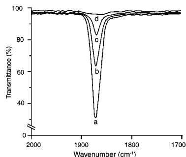
Figure 2. IR spectra of 3 in MeOH, before (a) and after 10 (b), 20 (c), and 30 min (d) of irradiation ( \lambda \geq 455 \text{ nm} ) at 20^\circ\text{C} .
